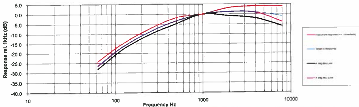
Overall Electro-Acoustic Frequency response - 'A' Weighted.
