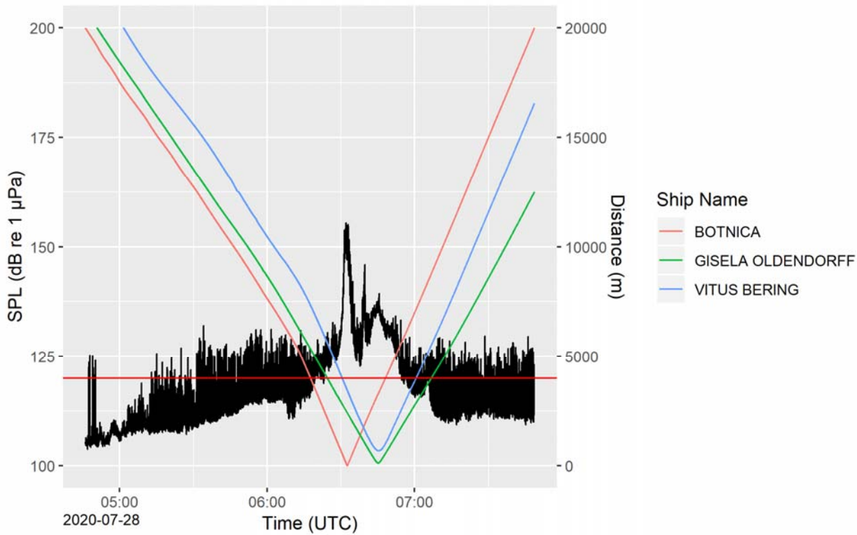
Figure B-30. AMAR-RI: SPL (left axis) as a function of time recorded while MSV Botnica transited through Eclipse Sound on 28 Jul 2020 coming to Milne Port, with 2 vessels in escort and 0/10 ice concentration. The distances (right axis) between the vessels and the AMAR is are plotted with color-coded lines. A solid red horizontal line marks the 120 dB re 1 \mu Pa SPL threshold for behavioural disturbance
