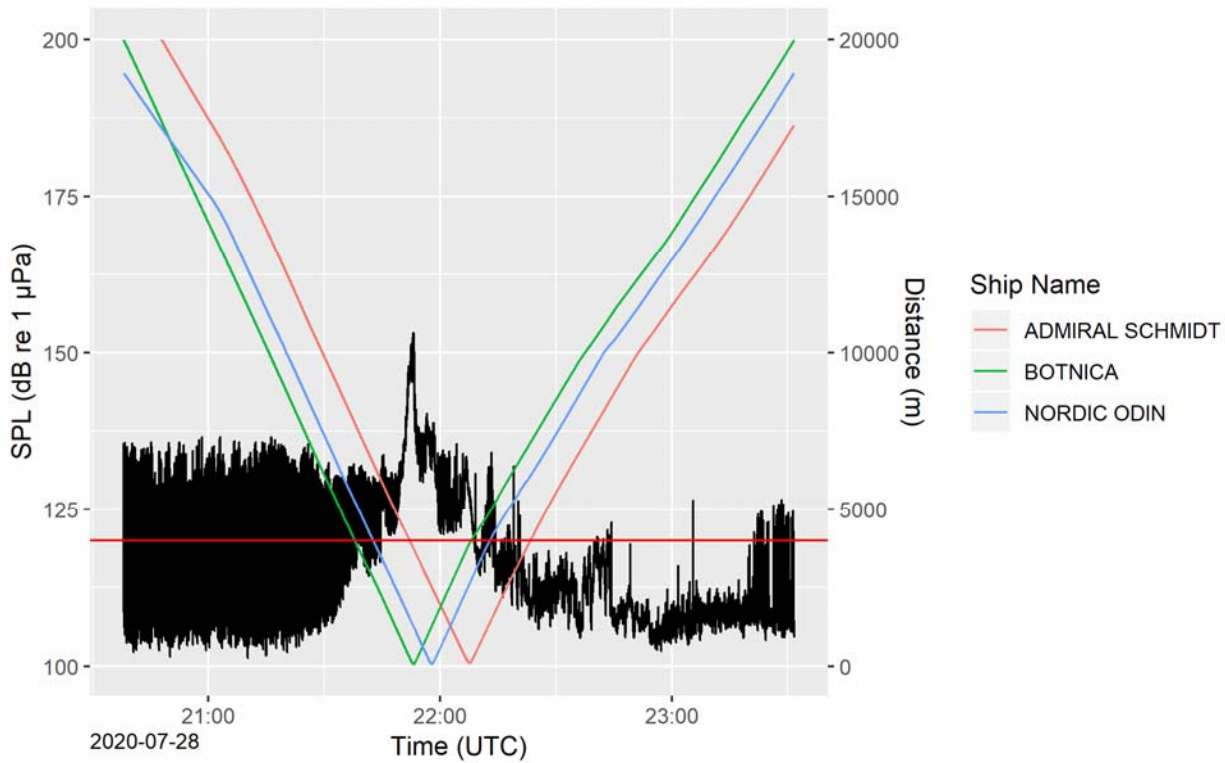
Figure B-31. AMAR-RI: SPL (left axis) as a function of time recorded while MSV Botnica transited through Eclipse Sound on 28 Jul 2020 leaving Milne Port, with 2 vessels in escort and 0/10 ice concentration. The distances (right axis) between the vessels and the AMAR is are plotted with color-coded lines. A solid red horizontal line marks the 120 dB re 1 \mu Pa SPL threshold for behavioural disturbance
