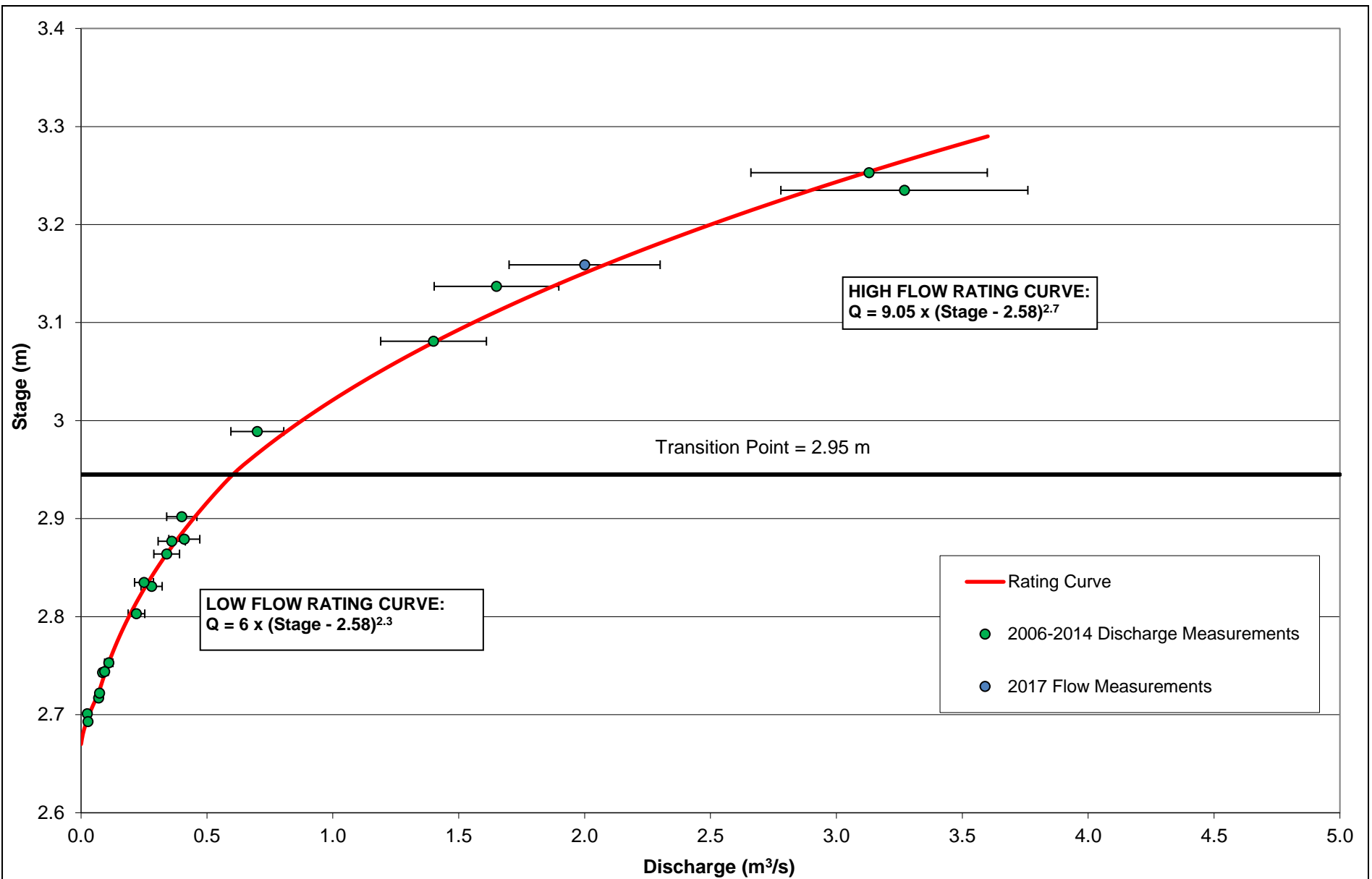
Figure 6 H07 - Mary River Tributary Rating Curve
