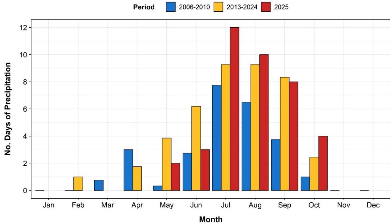
Figure 4:9: Milne Port monthly precipitation frequency (number of days experiencing precipitation) from 2006–2010, 2013–2023, and 2025.
