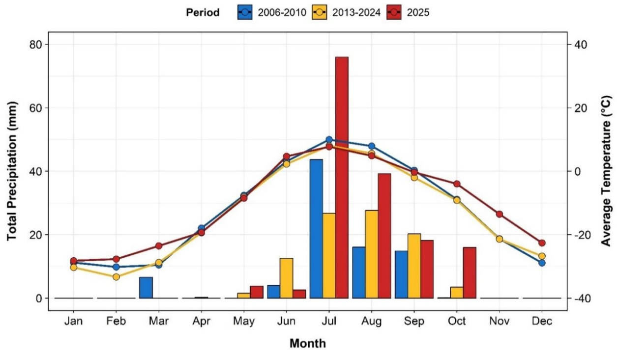
Figure 4:8: Milne Port monthly average air temperature (lines) and total precipitation (bars) from 2006–2010, 2013–2023, and 2025.
