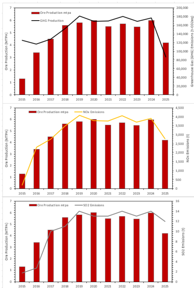
Figure 4:3: Greenhouse Gas (GHG), SO 2 and NO x Emissions relative to Ore Production
