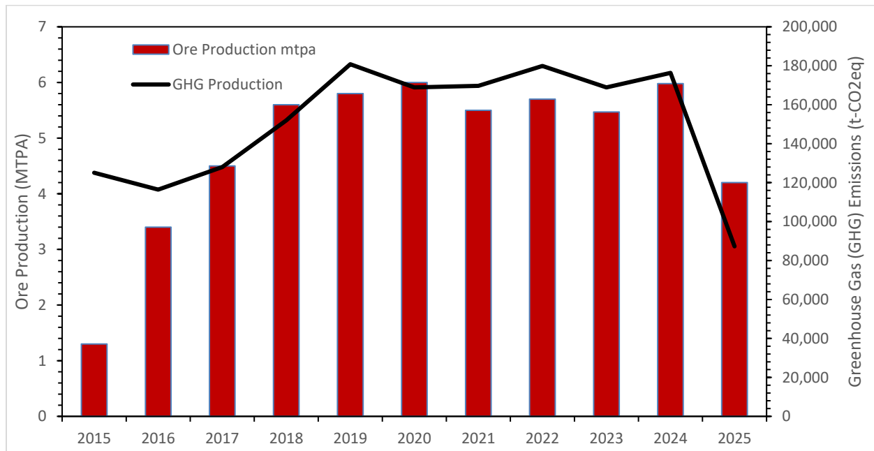
Figure 4:2: Greenhouse Gas (GHG) Emissions relative to Ore Production
